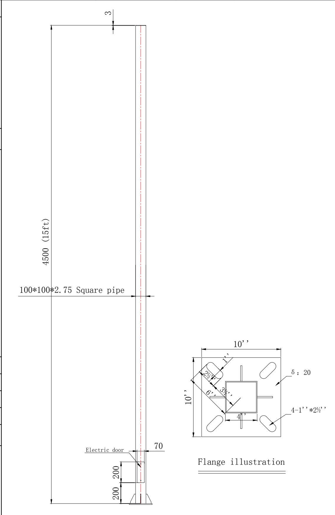
4.5 meter (15ft) street light structure
